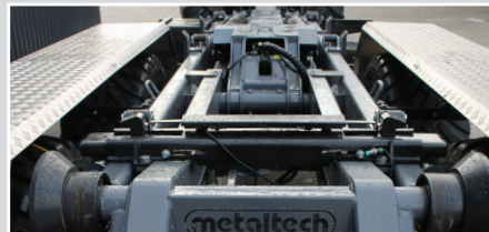
Hydraulisk containerlås
